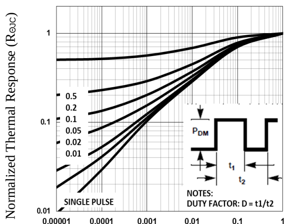
Fig.7 Normalized Transient Response
