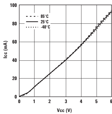
Figure 15. Supply Current vs. Voltage and Temperature.
