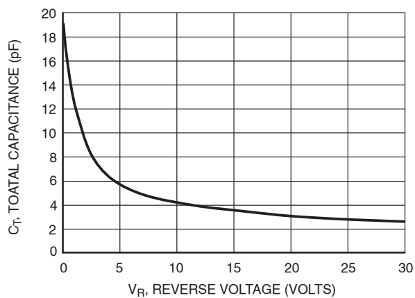
Figure 3. Total Capacitance
