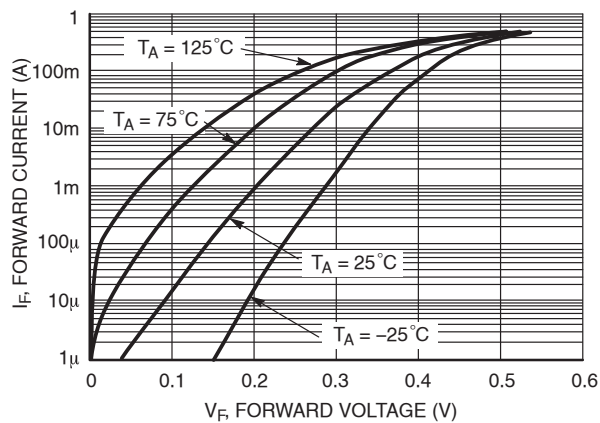
Figure 1. Forward Characteristics
