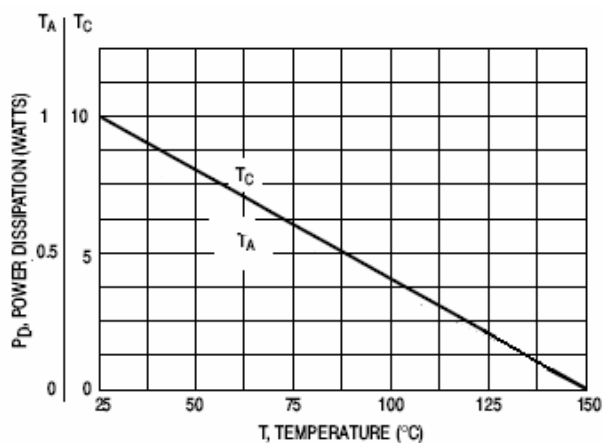
Figure 1. Power Derating
