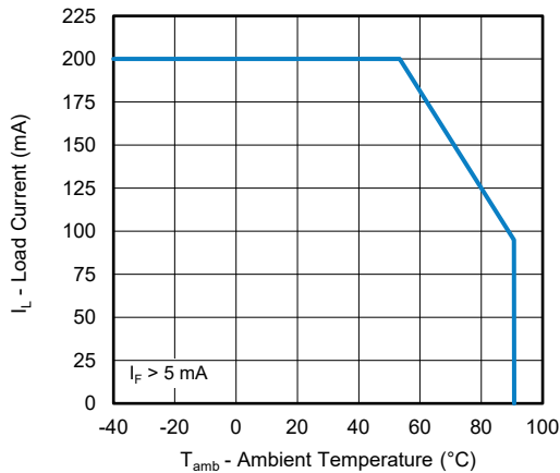
Fig. 8 Load Current vs. Ambient Temperature
