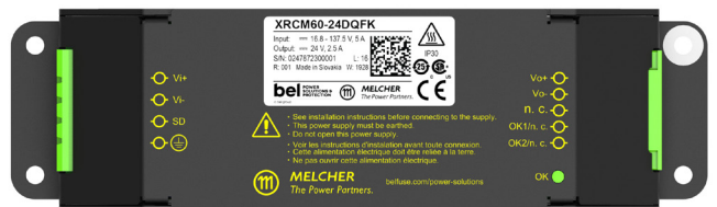
Fig. 14b Pin allocation of RCM60 (K option)
