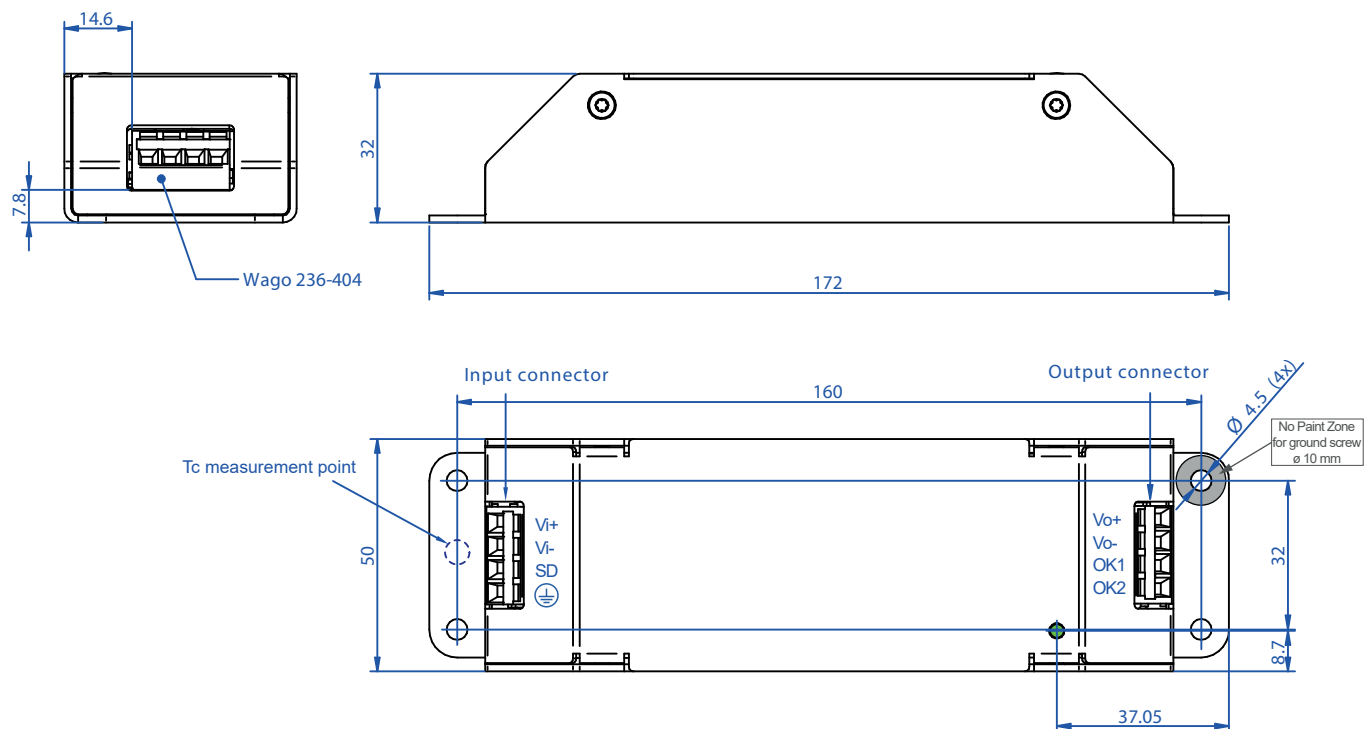
Fig. 12 Case of RCM60 with standard cage clamp terminals, Aluminum, EP-powder coated Weight approx. 350 g
