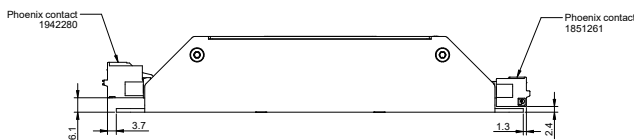
Fig. 14a Assembled input and output connector RCM60 (K option)
