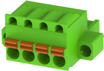
Fig. 15a Input plug for RCM60 with option K
