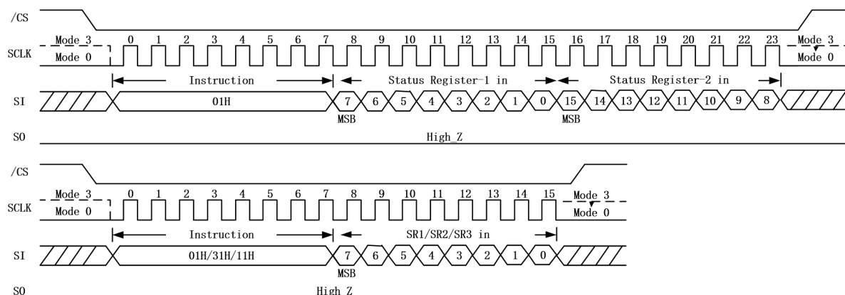
Figure 7.1.6. Write Status Register Instruction
