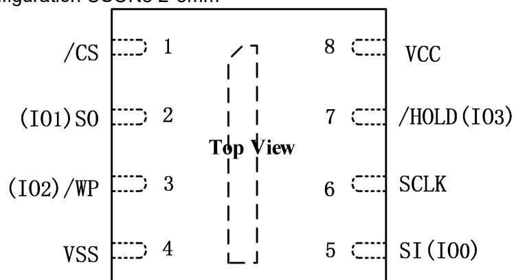
Figure 3. Pin Configuration USON8 2*3mm
