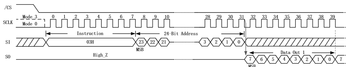
Figure 7.2.1. Read Data Instruction
