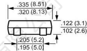
Dimensions in inches and (millimeters)
