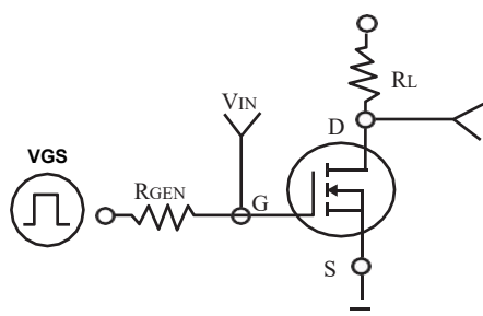
Figure 11a. Switching Test Circuit
