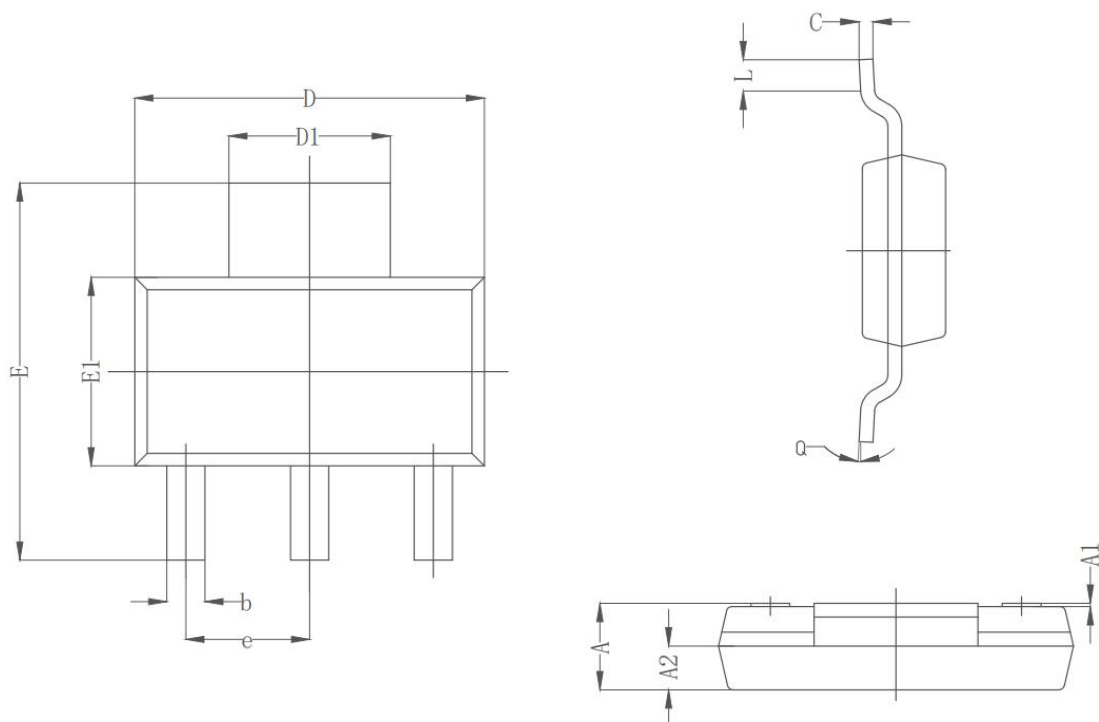
COMMON DIMENSION(MM)
