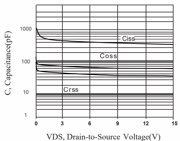
Fig.6 Capacitance
