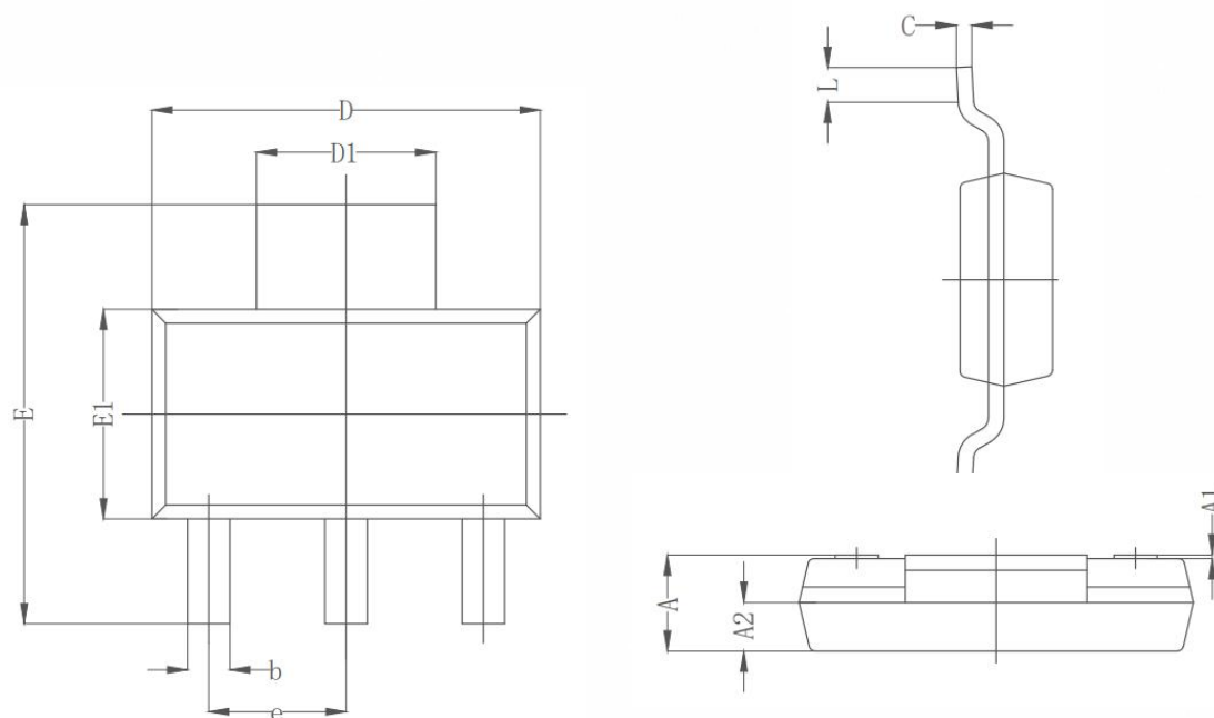
COMMON DIMENSION(MM)
