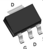
SOT-223 Pin Configuration
