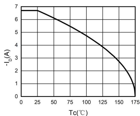
Figure 4. Drain Current
