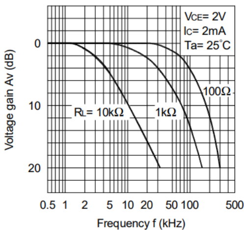
Fig.11 Frequency Response
