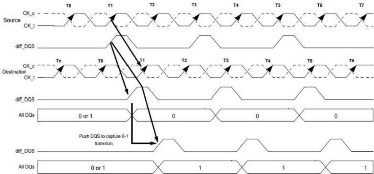
Figure 4 Write Leveling Concept
