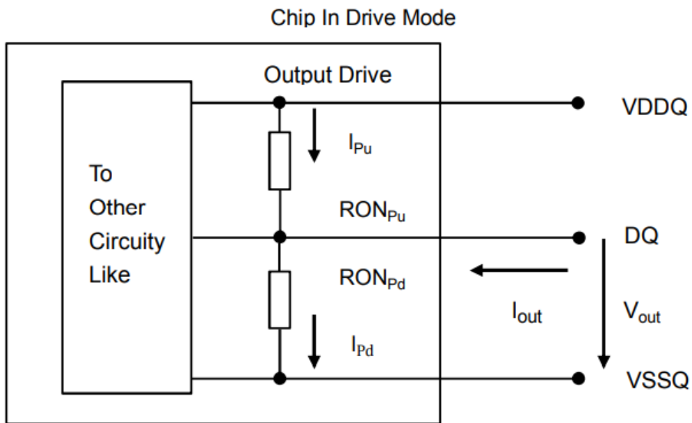
Figure 19 Output driver
