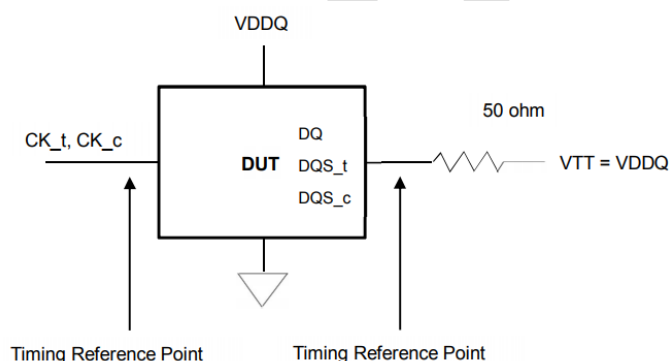
Figure 26 Reference Load for AC Timing and Output Slew Rate
