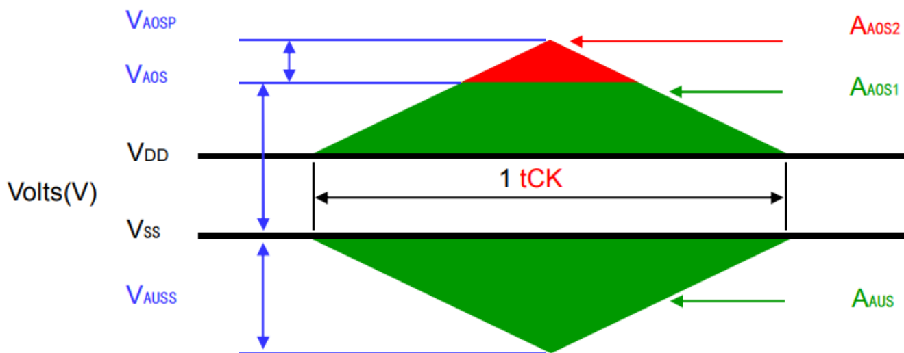
Figure 8 Address, Command and Control Overshoot and Undershoot Definition
