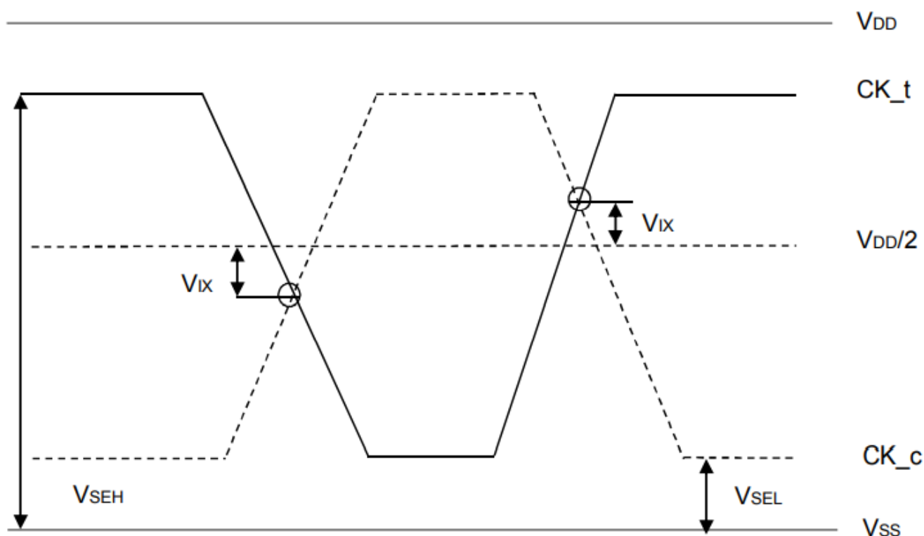
Figure 13 VIX Definition (CK)
