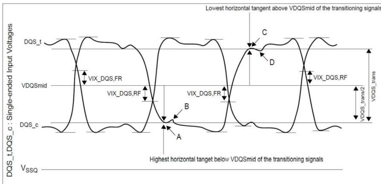
Figure 17 Vix Definition (DQS)
