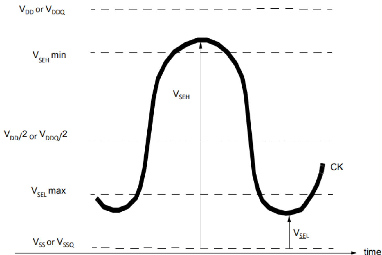
Figure 7 Single-ended requirement for differential signals
