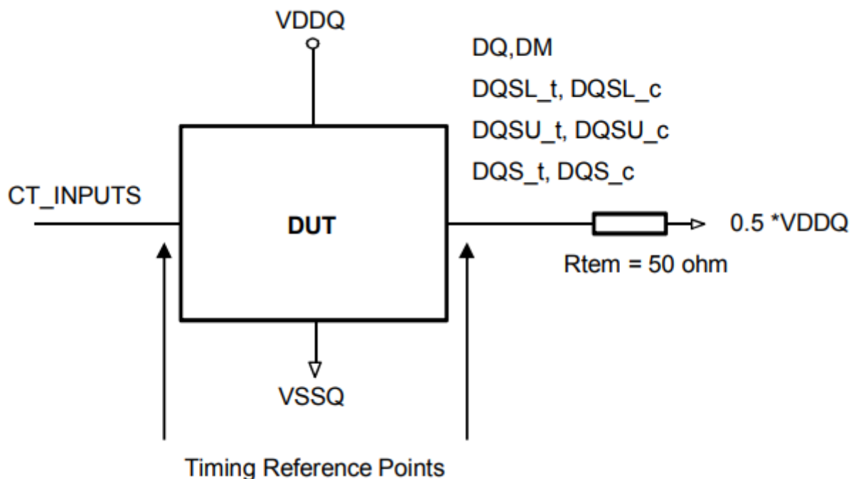
Figure 23 Connectivity Test Mode Timing Reference Load
