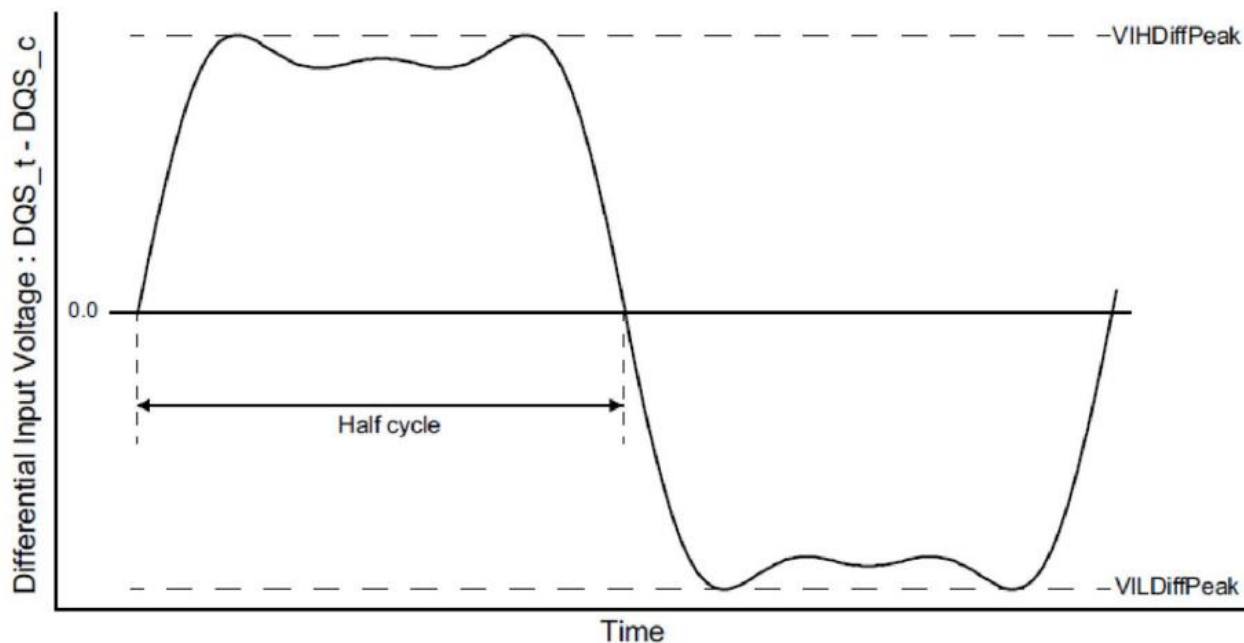
Figure 15 Definition of differential DQS Signal AC-swing Level
