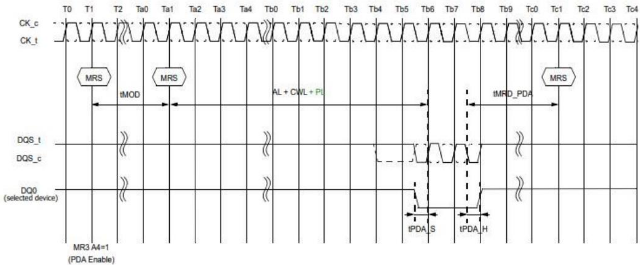
Figure 3 PDA using Burst Chop 4
