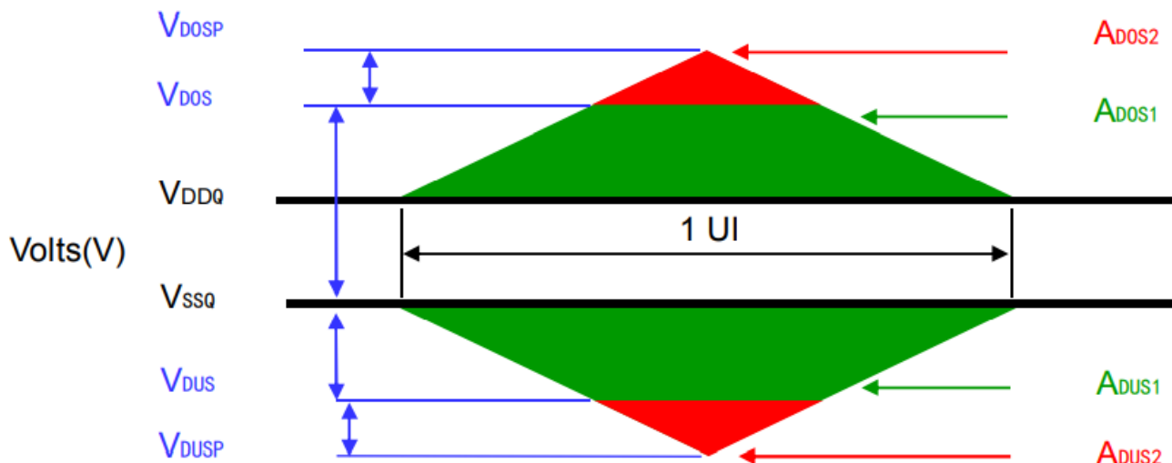
Figure 10 Data, Strobe and Mask Overshoot and Undershoot Definition
