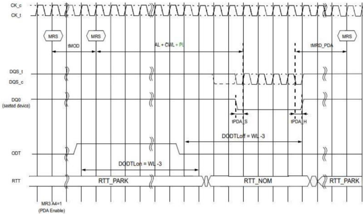
Figure 1 MRS w/ per DRAM addressability (PDA) issuing before MRS
