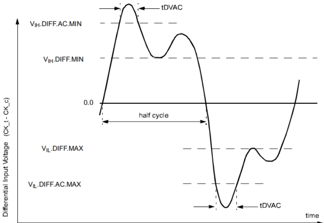
Figure 6 Definition of differential ac-swing and "time above ac-level" tDVAC
