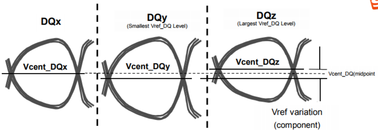
Figure 28 Vcent_DQ Variation to Vcent_DQ(midpoint)
