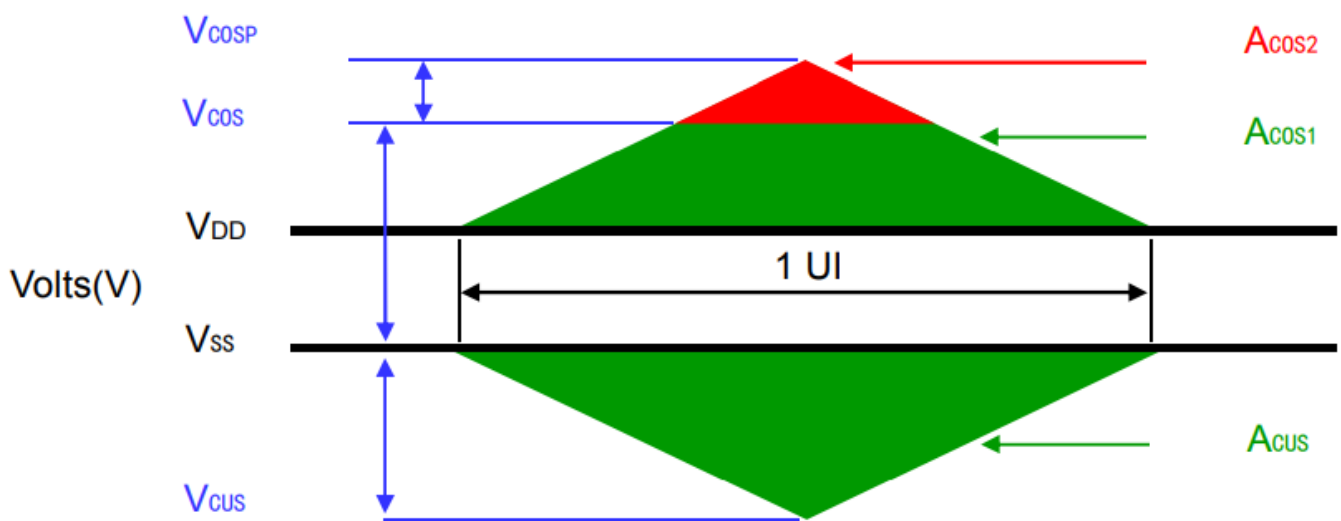
Figure 9 Clock Overshoot and Undershoot Definition
