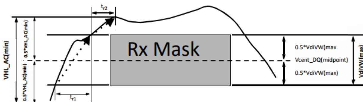
Figure 30 Slew Rate Conditions For Rising Transition
