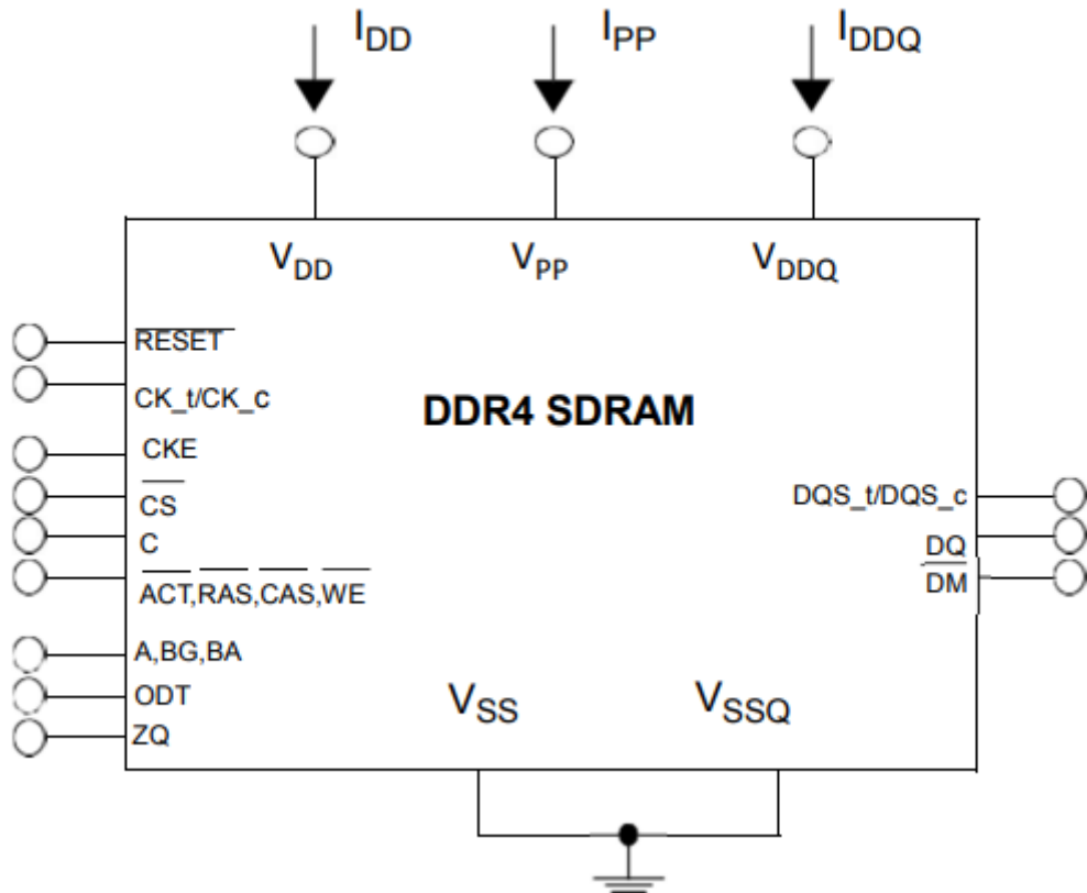
Figure 24 Measurement Setup and Test Load for IDD, IPP and IDDQ Measurements
