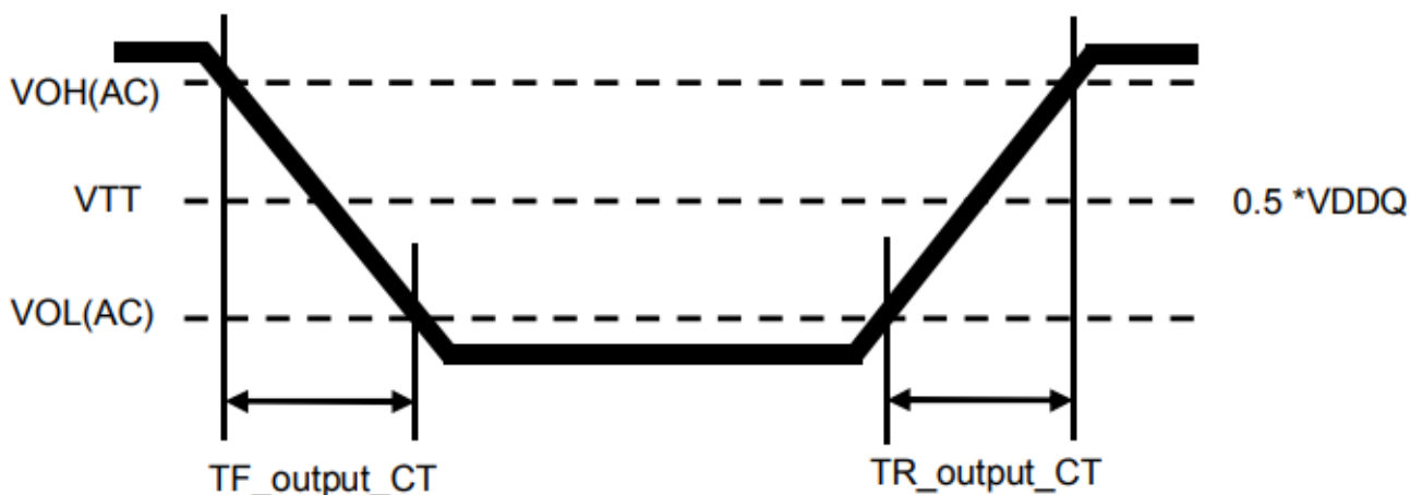
Figure 22 Output Slew Rate Definition of Connectivity Test Mode
