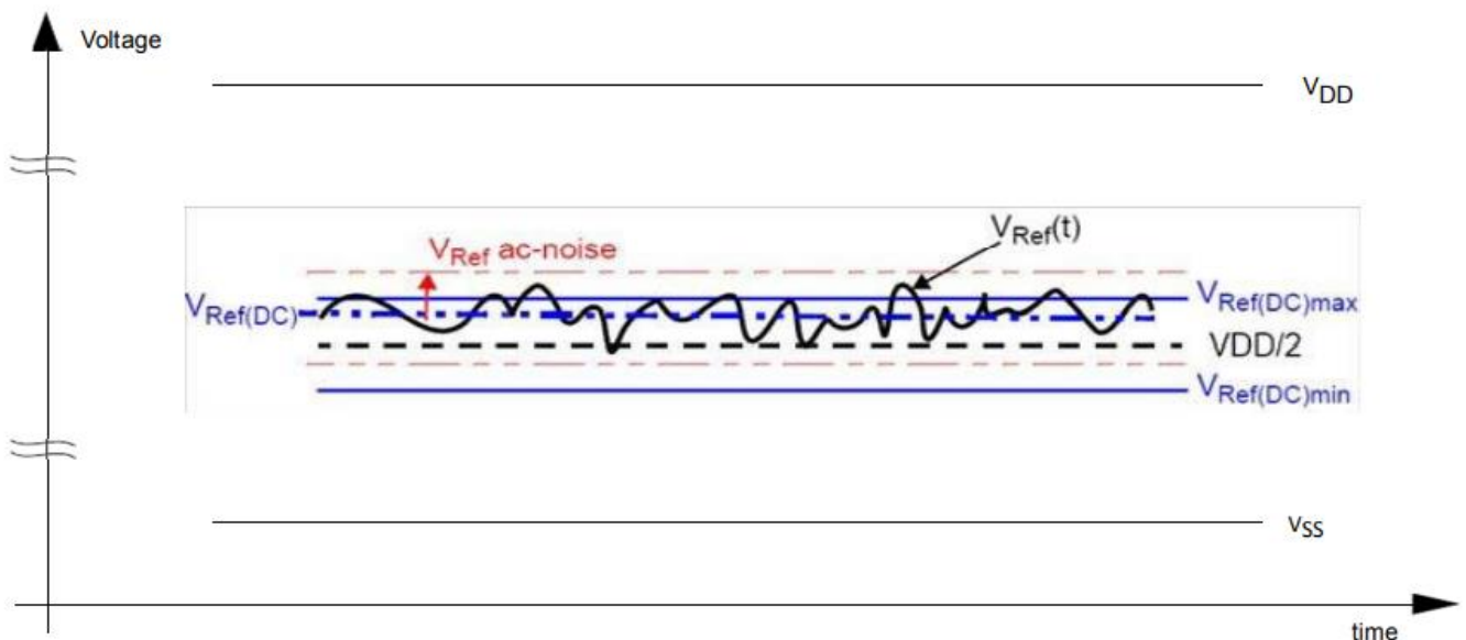
Figure 5 Illustration of V_{REF}(DC) tolerance and V_{REF} AC-noise limits
