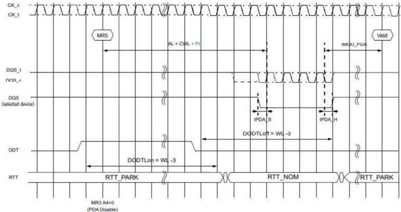
Figure 2 MRS w/ per DRAM addressability (PDA) Exit
