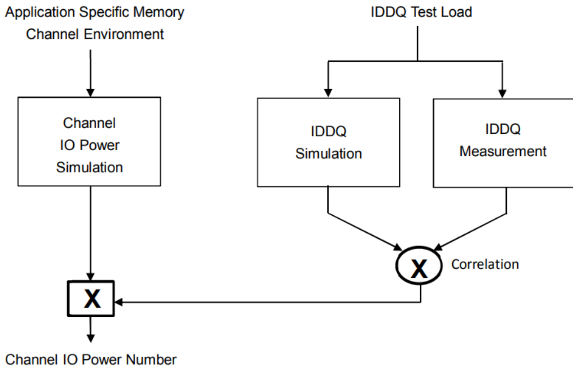
Figure 25 Correlation from simulated Channel IO Power to actual Channel IO Power supported by IDDQ Measurement
