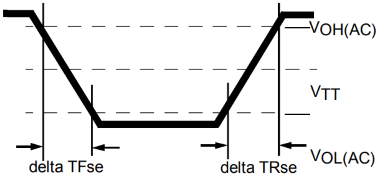
Figure 20 Single-ended Output Slew Rate Definition
