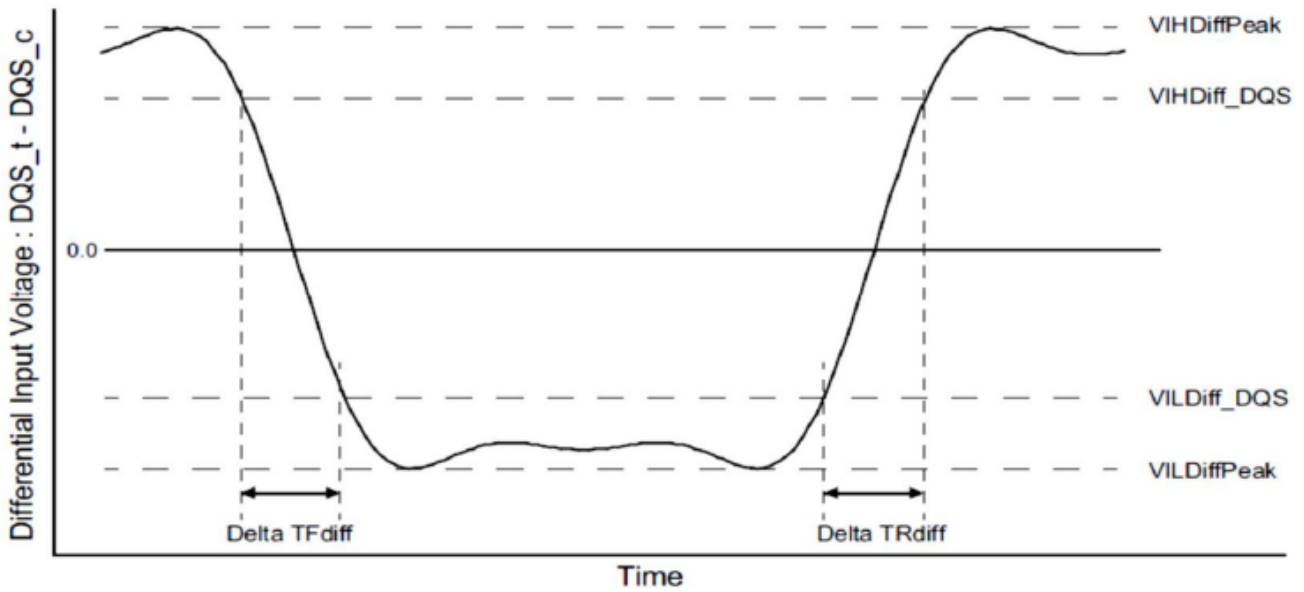
Figure 18 Differential Input Slew Rate Definition for DQS_t, DQS_c
