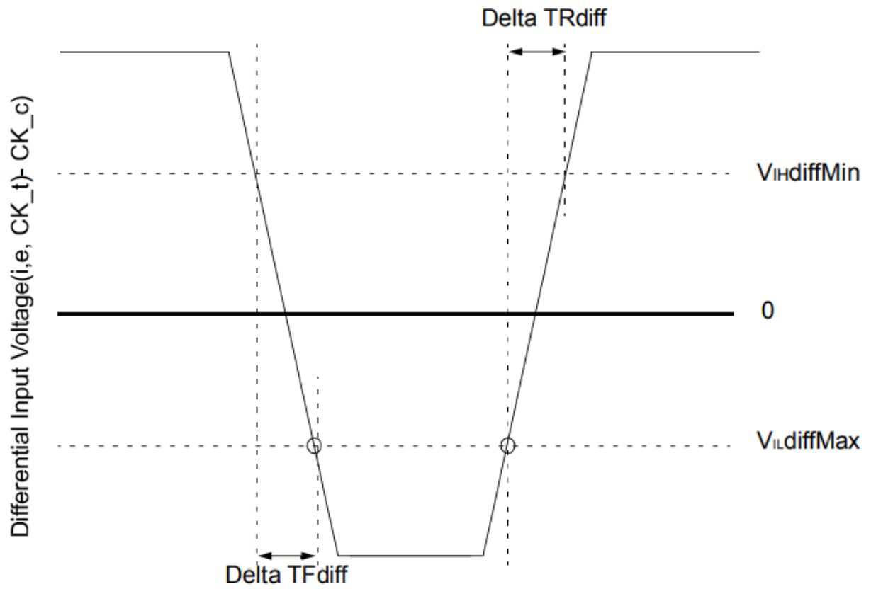
Figure 11 Differential Input Slew Rate Definition for CK t , CK c
