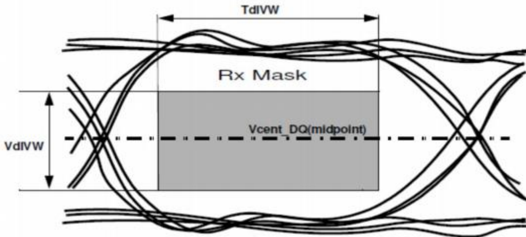
Figure 27 DQ Receiver(Rx) compliance mask
