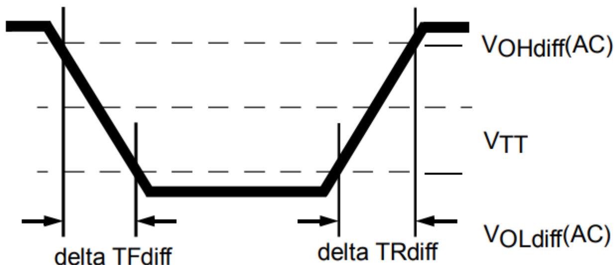
Figure 21 Differential Output Slew Rate Definition
