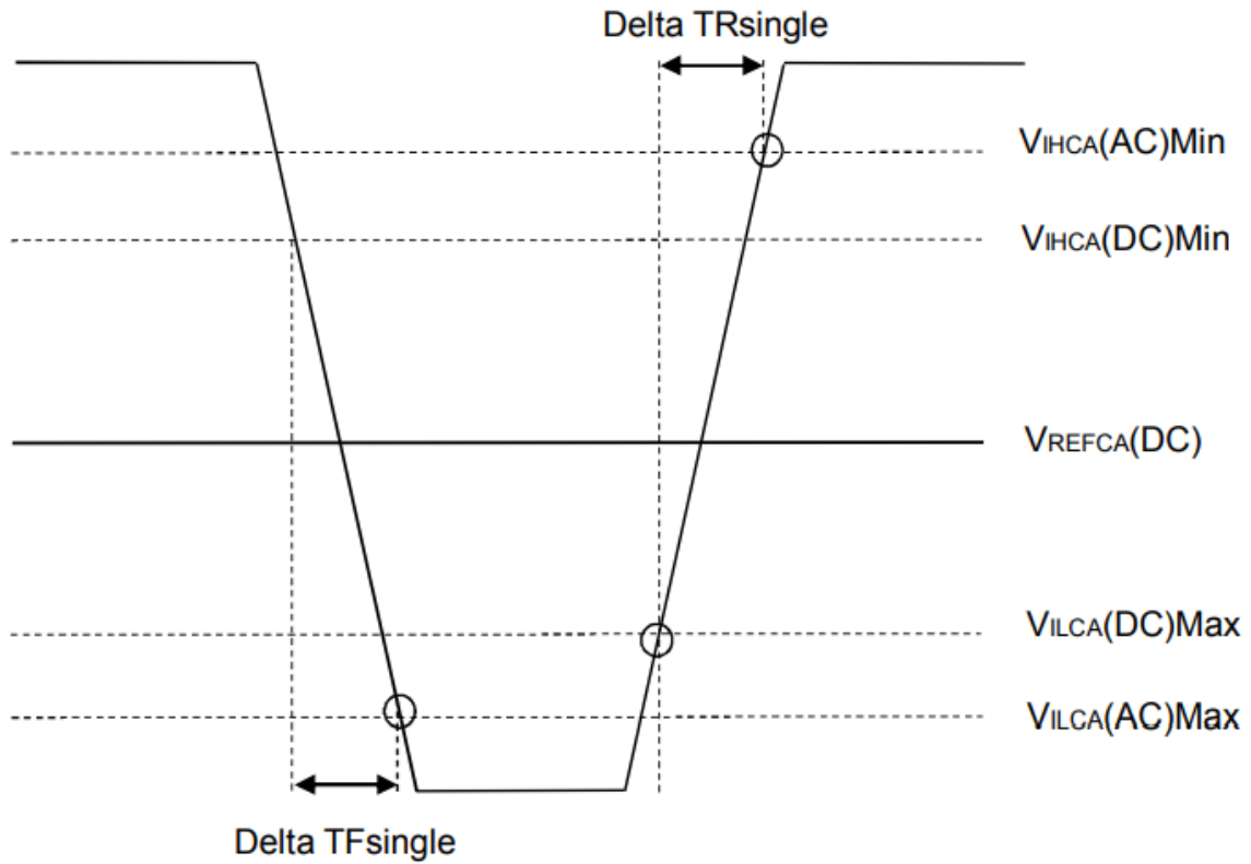
Figure 12 Single-ended Input Slew Rate definition for CMD and ADD
