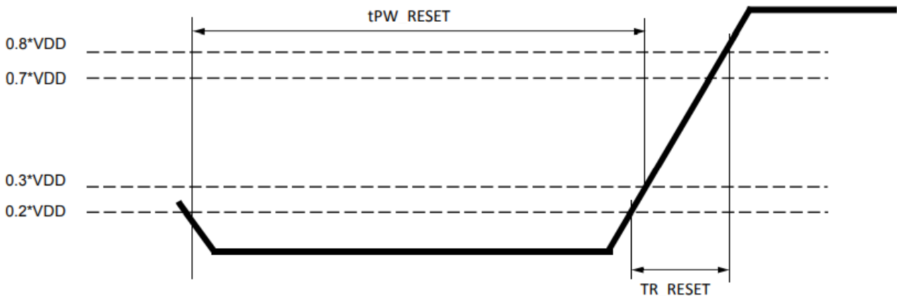
Figure 14 RESET_n Input Slew Rate Definition
