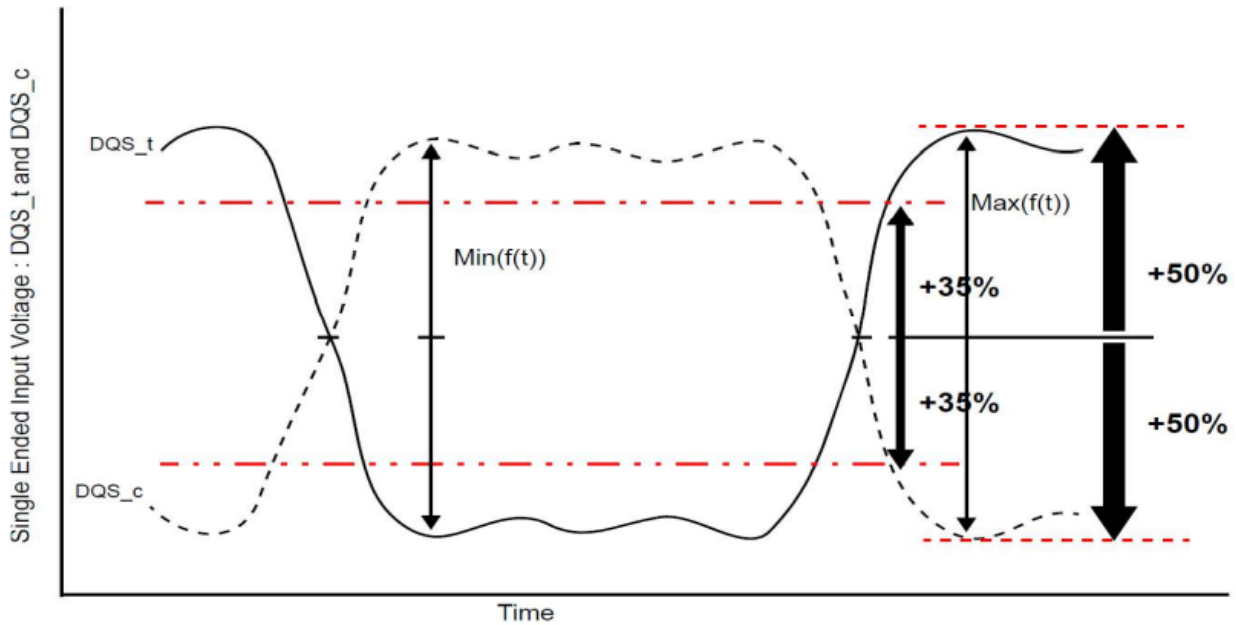
Figure 16 Definition of differential DQS Peak Voltage and range of exempt nonmonotonic signaling
