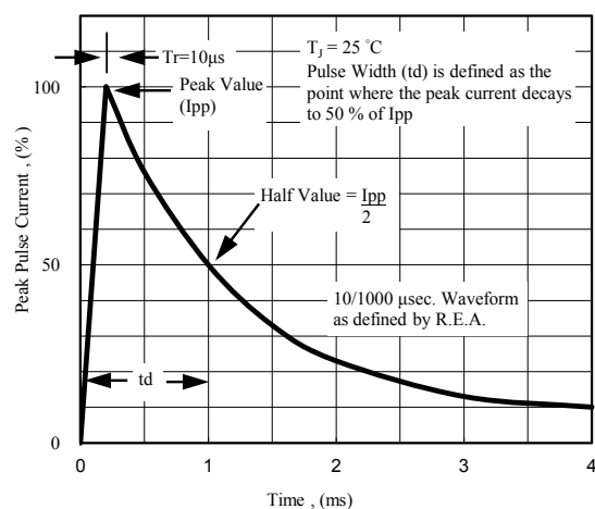
Fig. 5 - Pulse Waveform
