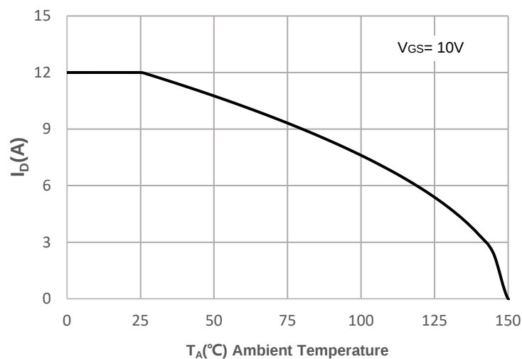
Figure 10: Maximum Continuous Drian Current vs. Ambient Temperature
