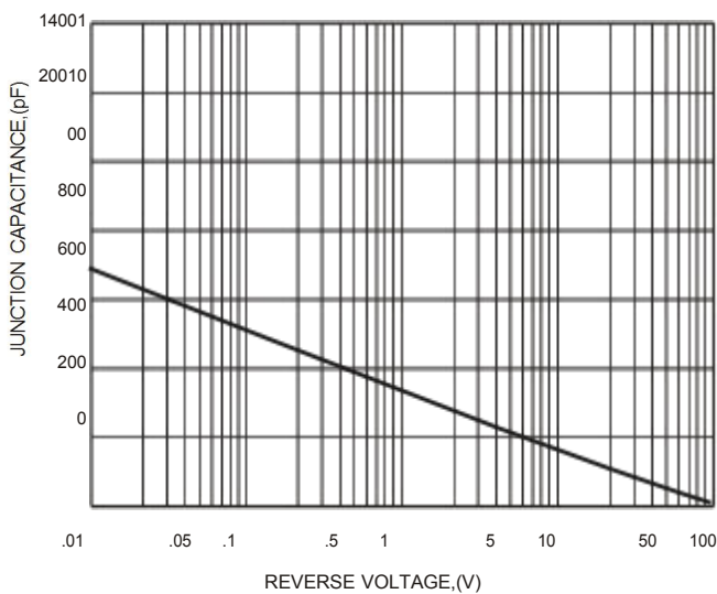
FIG.4-TYPICAL JUNCTION CAPACITANCE
