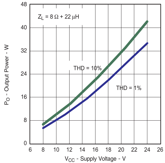
OUTPUTPOWER vs SUPPLYVOLTAGE(STEREO)
