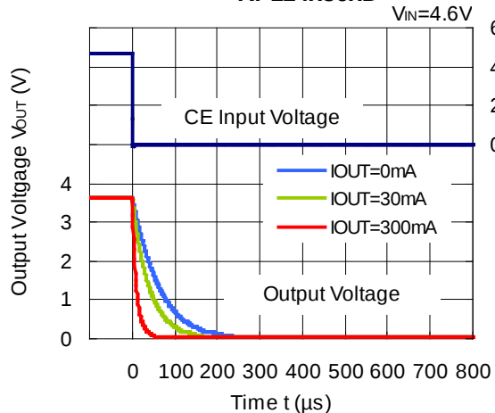
RP114x36xD
