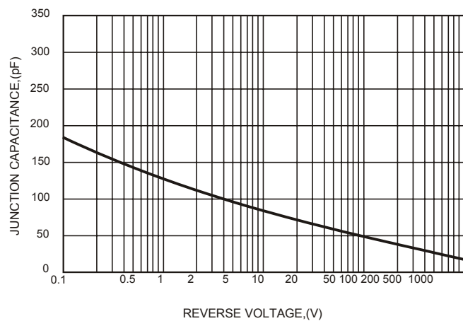
FIG.5-TYPICAL JUNCTION CAPACITANCE
