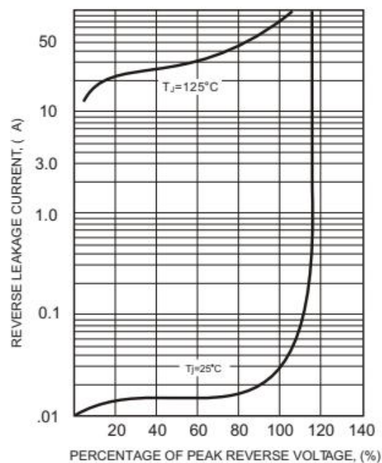
FIG.4-TYPICAL REVERSE CHARACTERISTICS
