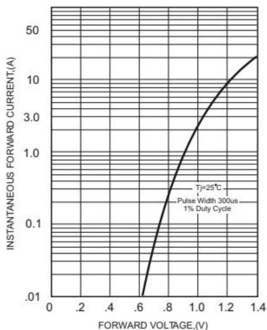
FIG.3-TYPICAL FORWARD CHARACTERISTICS
