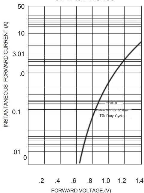
FIG.3-TYPICAL FORWARD CHARACTERISTICS
