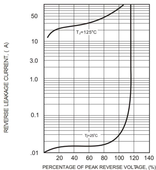
FIG.4-TYPICAL REVERSE CHARACTERISTICS
