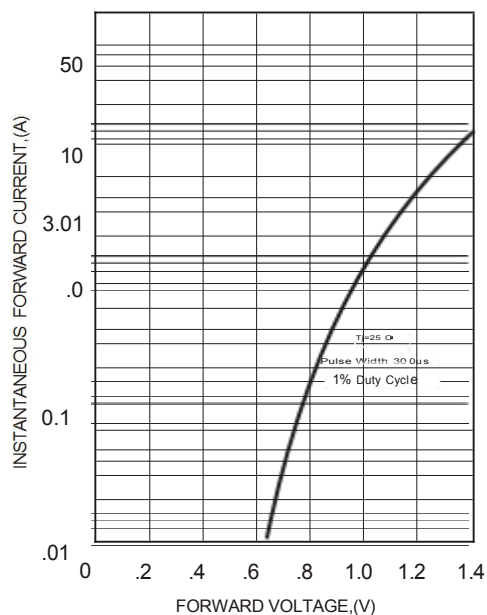
FIG.3-TYPICAL FORWARD CHARACTERISTICS
