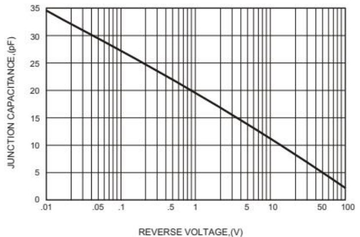
FIG.5-TYPICAL JUNCTION CAPACITANCE
