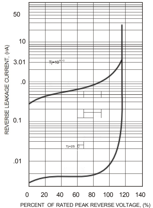
FIG.4-TYPICAL REVERSE CHARACTERISTICS
