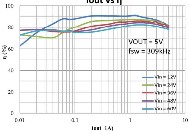
I_{OUT} vs \eta
