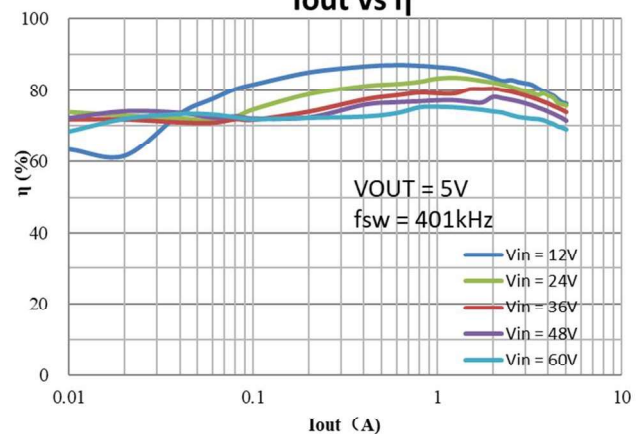
I_{OUT} vs \eta
