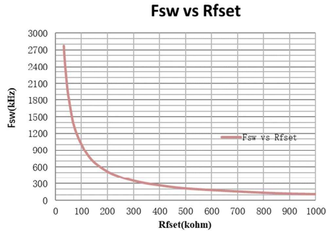
Figure 2 Fsw vs Rfset
