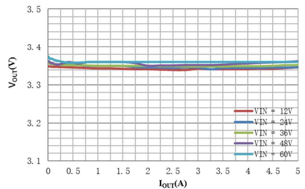
I_{OUT} vs V_{OUT}
