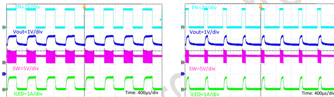
PWM signal: 2kHz frequency, 50% duty
