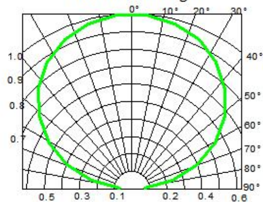
Radiation angle
