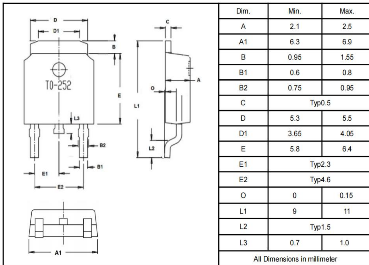
TO-252
