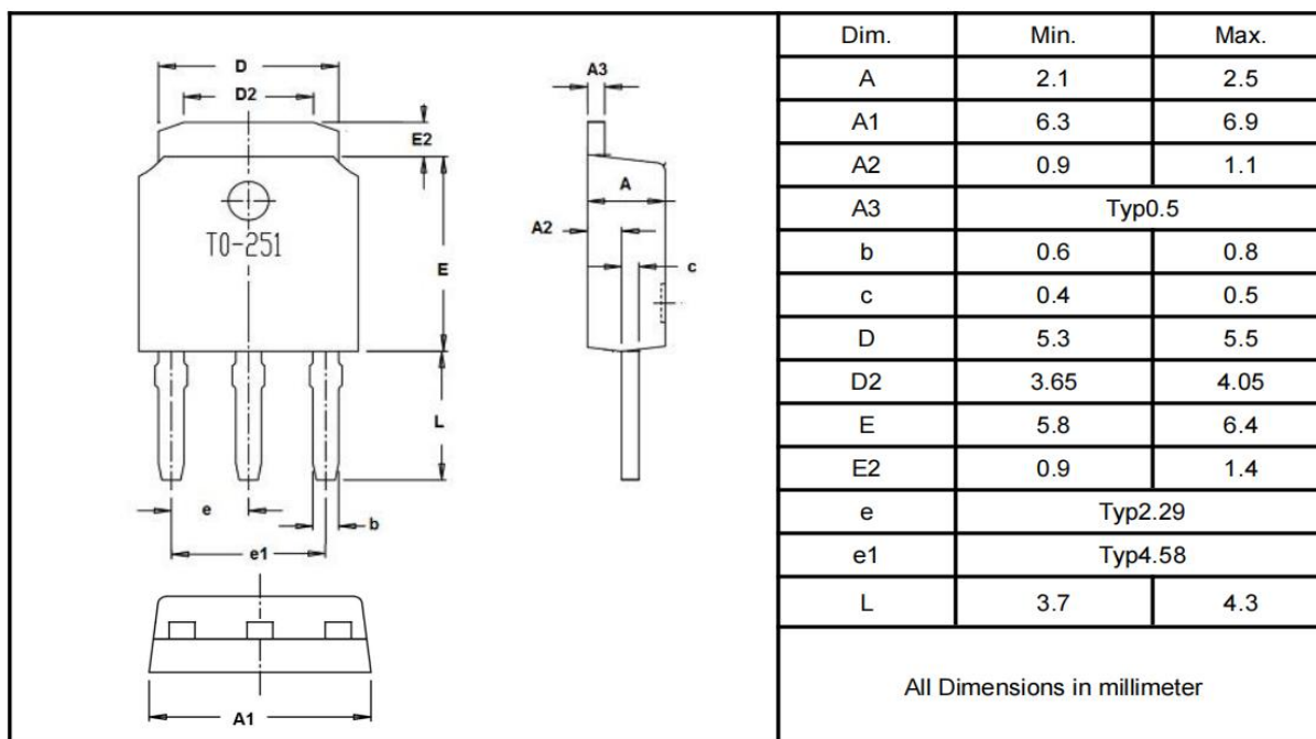
TO-251
