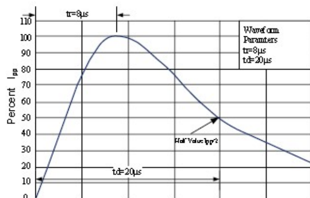
Figure 5: Pulse Waveform
