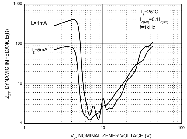
Fig.6 Effect of Zener Voltage on Zener Impedance
