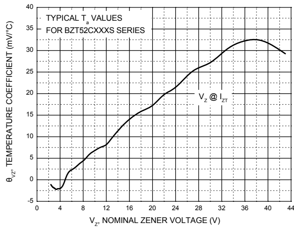
Fig.3 Temperature Coefficients
