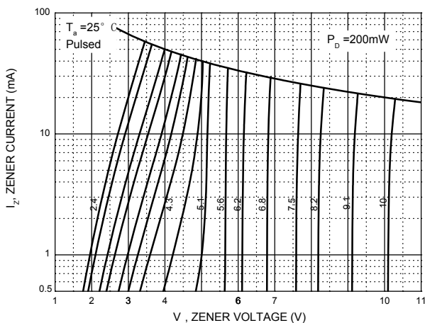
Fig.1 Zener Characteristics (V Z Up to 10 V)
