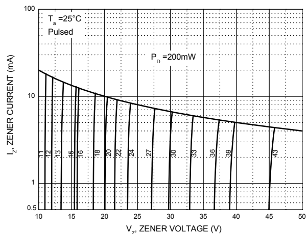
Fig.2 Zener Characteristics (11 V to 43 V)
