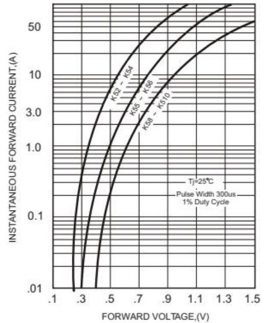
FIG.2-TYPICAL FORWARD CHARACTERISTICS
