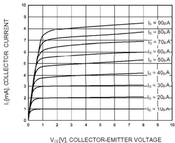
Static Characteristic
