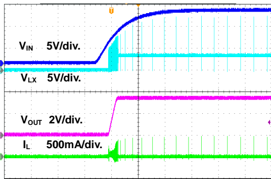
Figure 12. Startup Through Power Supply Waveform
