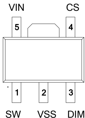
SOT89-5
