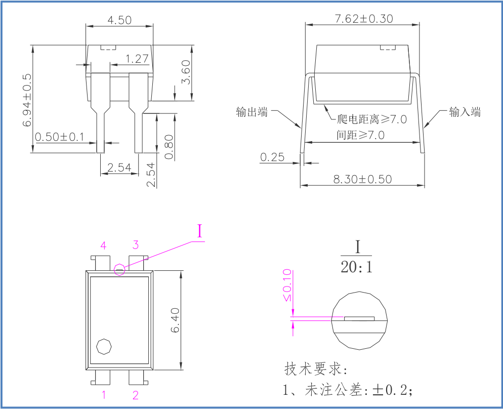
图 3 MT-AQY214EH外形尺寸 Figure 3- The dimensions of MT-AQY214EH
