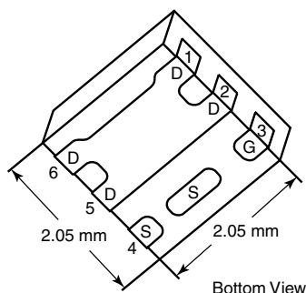
DFN2X2
