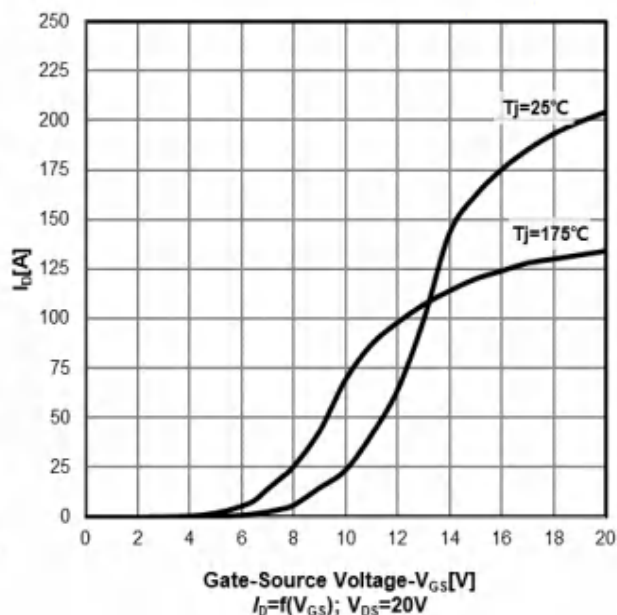
Transfer characteristics
