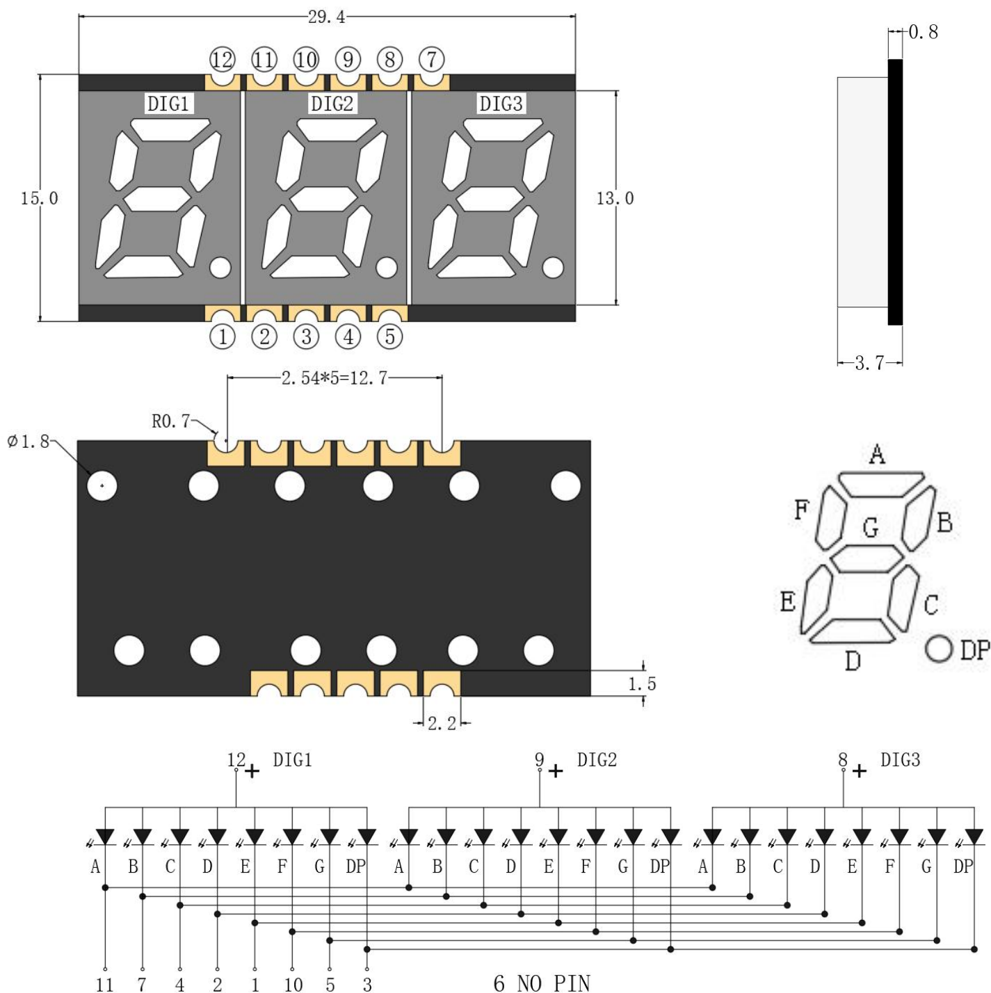
Figure Size & Circuit Principle Diagram : 29.4mm×15mm×3.7mm
