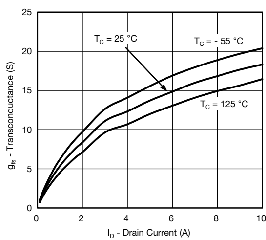
Transconductance
