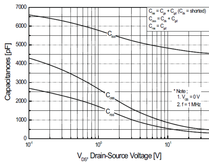
Figure 5. Capacitance Characteristics
