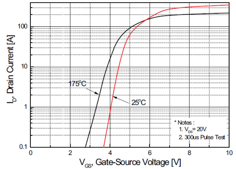
Figure 2. Transfer Characteristics
