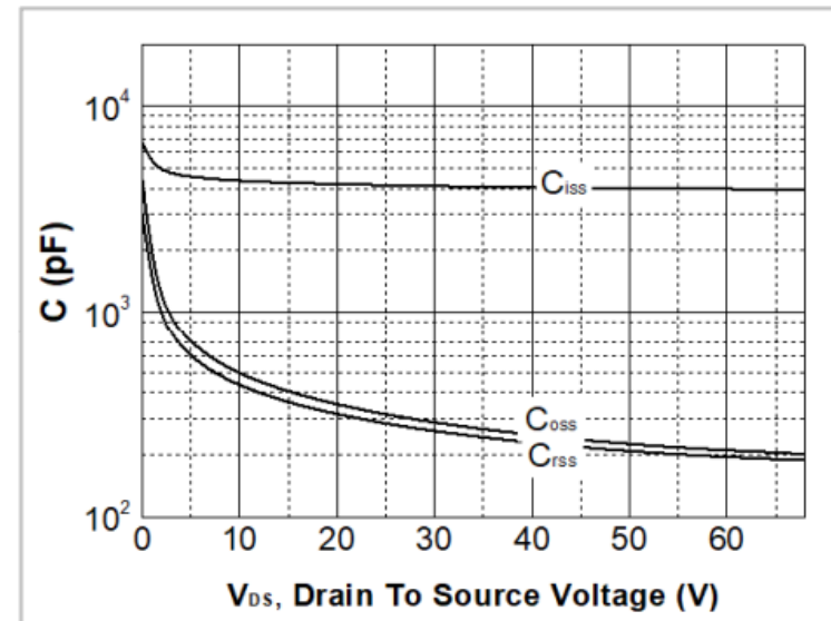
Fig. 8. Capacitance Characteristics
