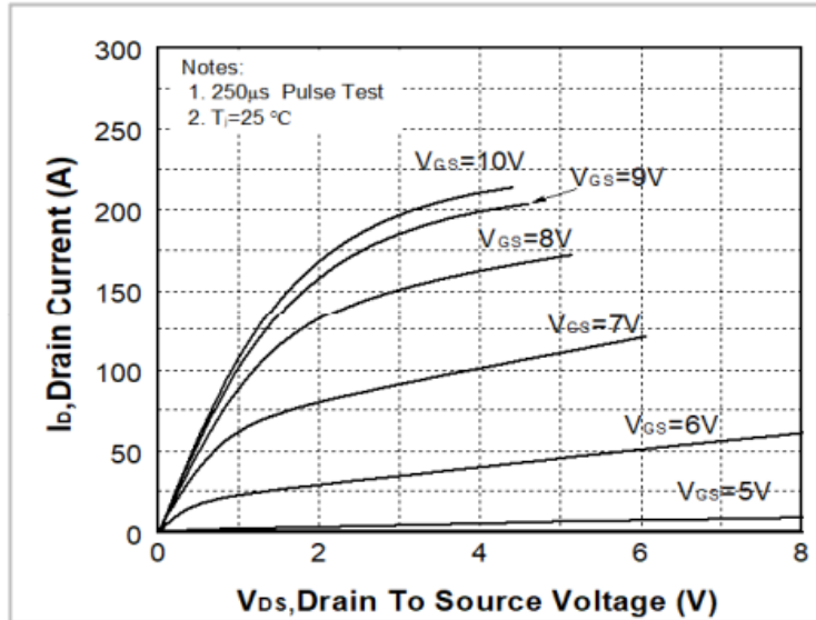
Fig. 1. On-state characteristics
