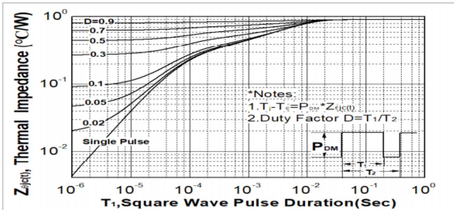
Fig. 11. Transient thermal response curve
