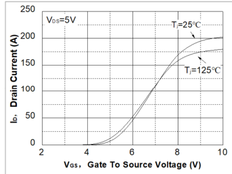
Fig. 2. Transfer Characteristics
