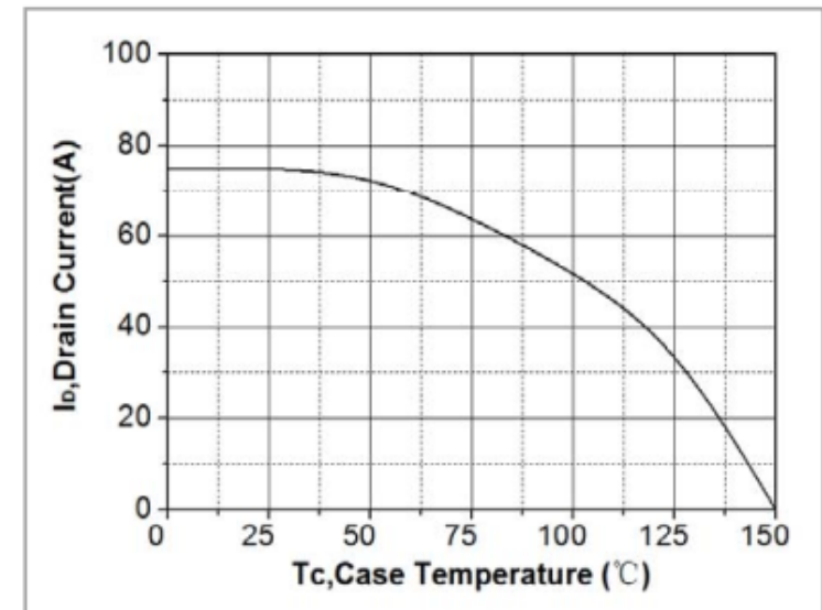
Fig. 10. Maximum drain current vs. case temperature
