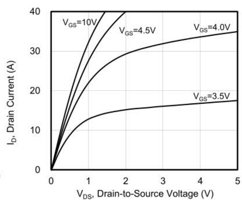
Figure 4. Typical output Characteristics
