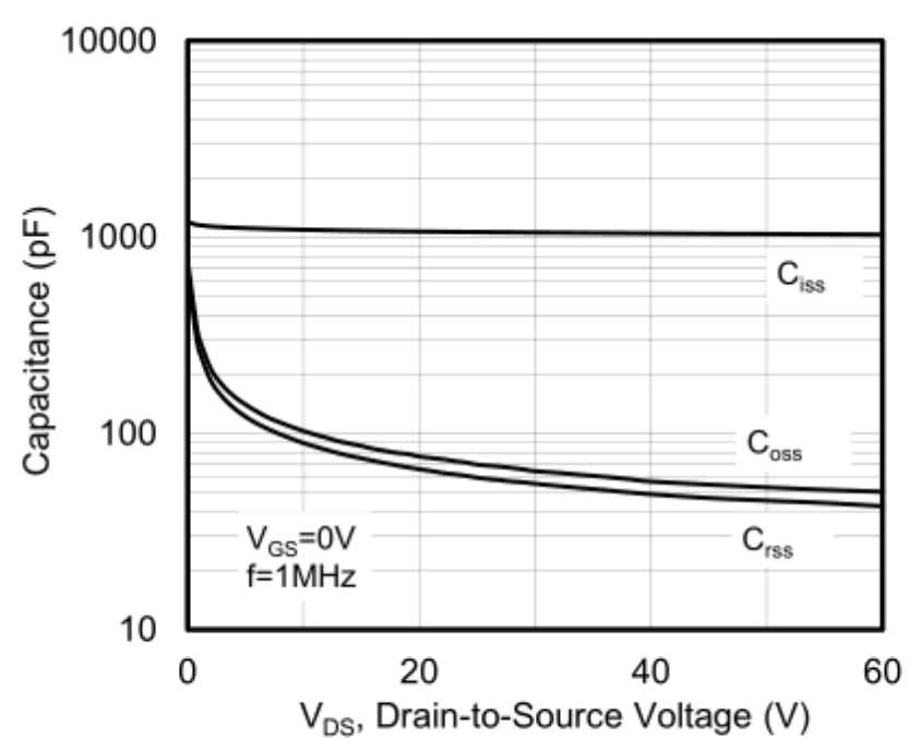
Figure 12. Capacitance Characteristics
