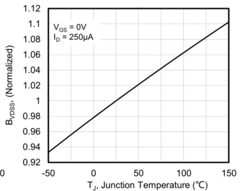
Figure 11. Normalized Breakdown Voltage vs Junction Temperature
