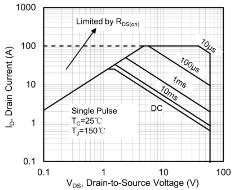
Figure 1. Maximum Safe Operating Area
