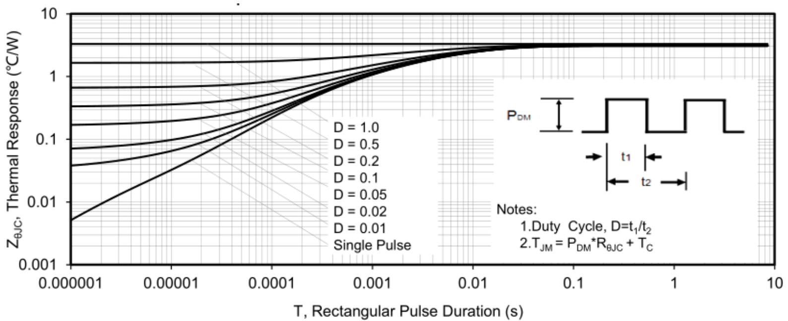
Figure 5. Maximum Effective Thermal Impedance, Junction to Case
