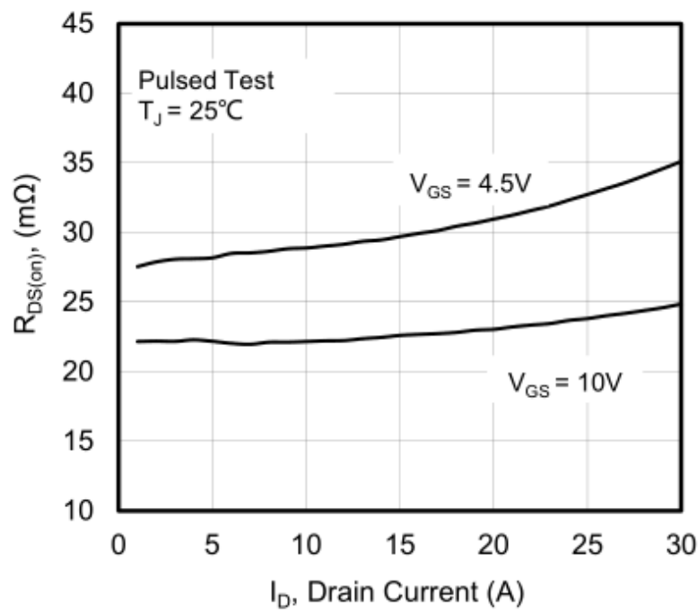
Figure 8. Drain-to-Source On Resistance vs Drain Current
