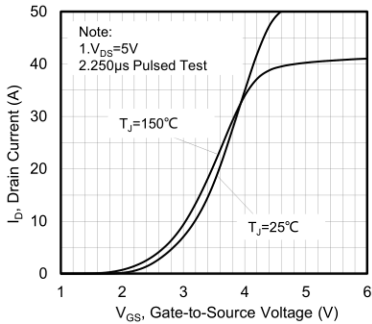
Figure 6. Typical Transfer Characteristics
