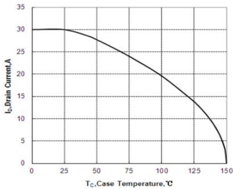
Figure 3. Maximum Continuous Drain Current vs. Case Temperature
