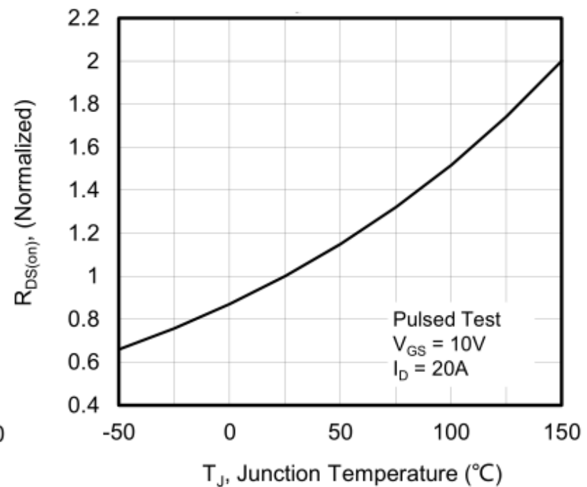
Figure 9. Normalized On Resistance vs Junction Temperature
