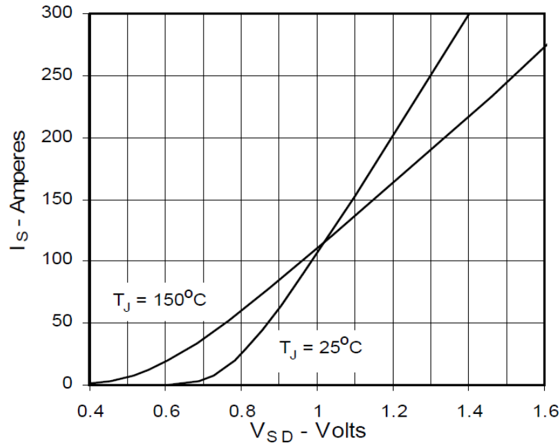
Fig. 9. Source Current vs. Source-To-Drain Voltage
