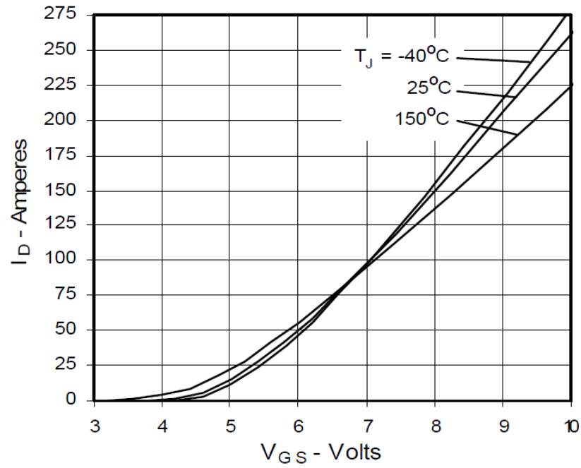
Fig. 7. Input Admittance
