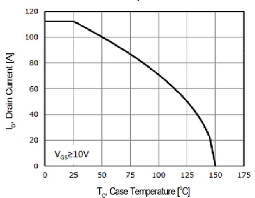
Fig. 6. Drain Current vs. Case Temperature
