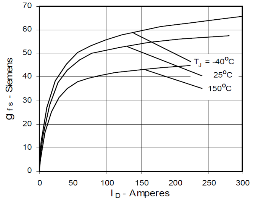
Fig. 8. Transconductance
