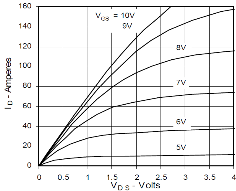
Fig. 3. Output Characteristics @ 150°C
