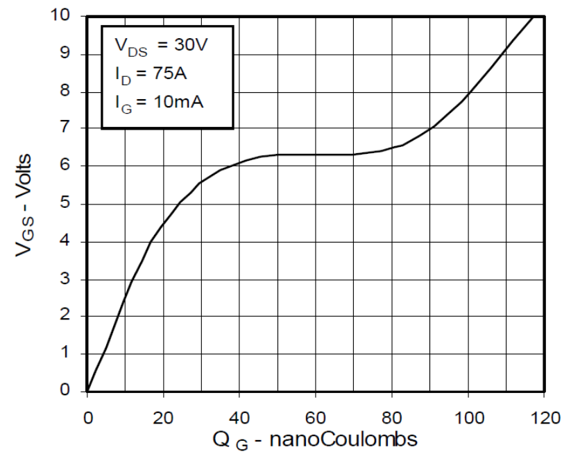
Fig. 10. Gate Charge
