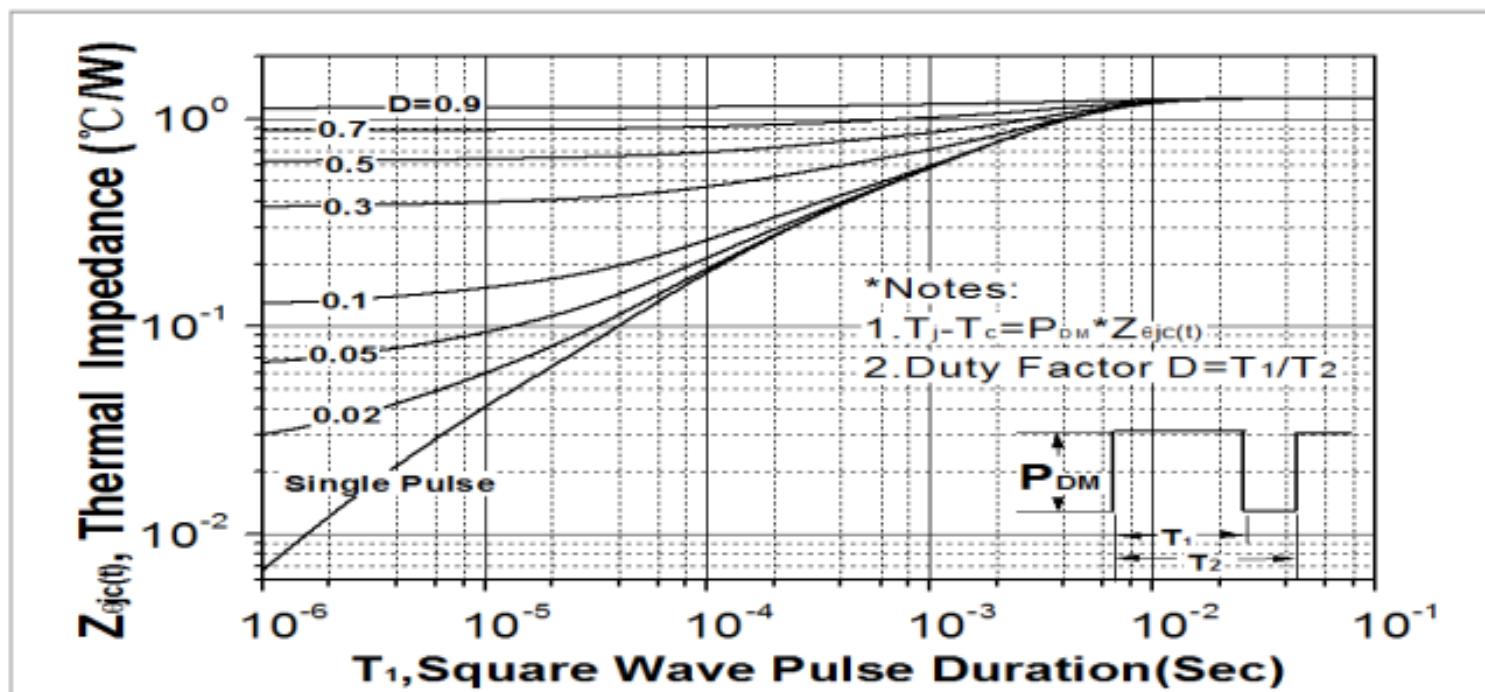
Fig. 11. Transient thermal response curve
