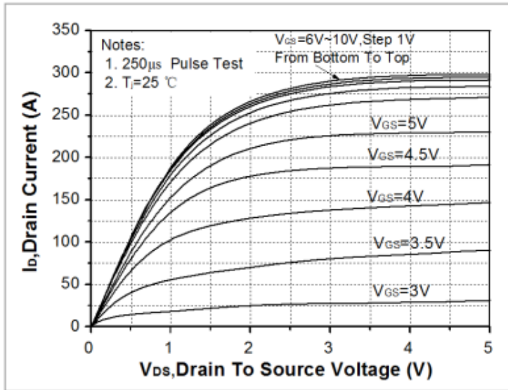
Fig. 1. On-state characteristics
