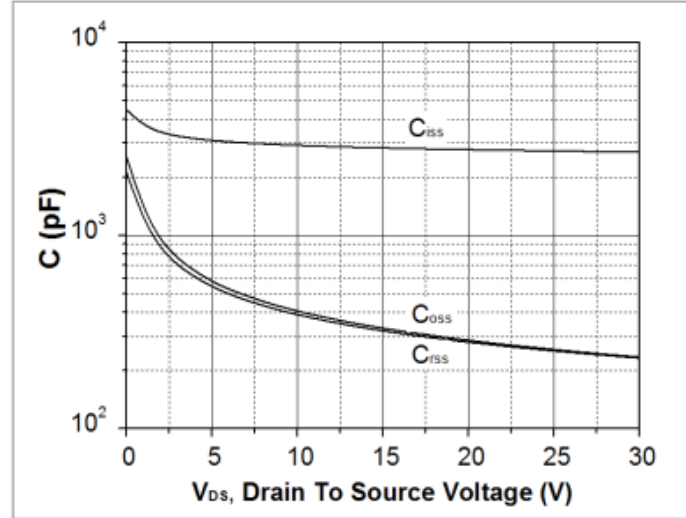
Fig. 8. Capacitance Characteristics
