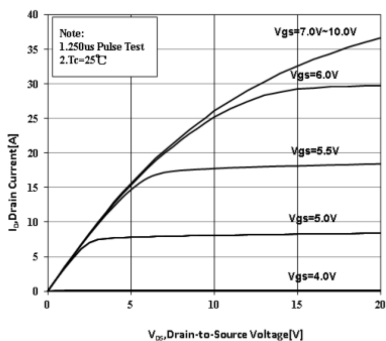
Figure 4 Typical Output Characteristics
