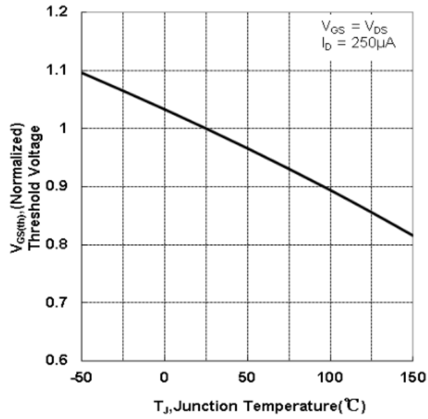
Figure 10 Typical Threshold Voltage vs Junction Temperature
