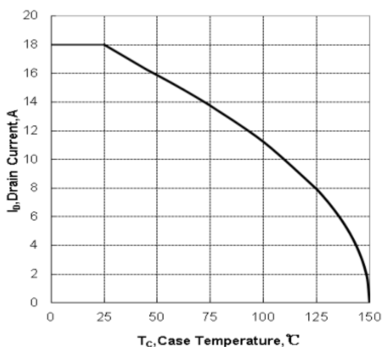
Figure 3 Maximum Continuous Drain Current vs Case Temperature
