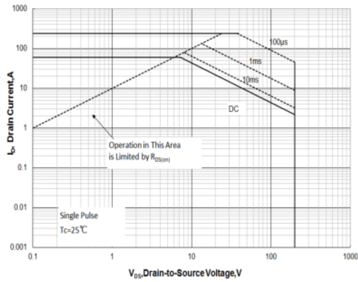
Figure 1 Maximum Forward Bias Safe Operating Area
