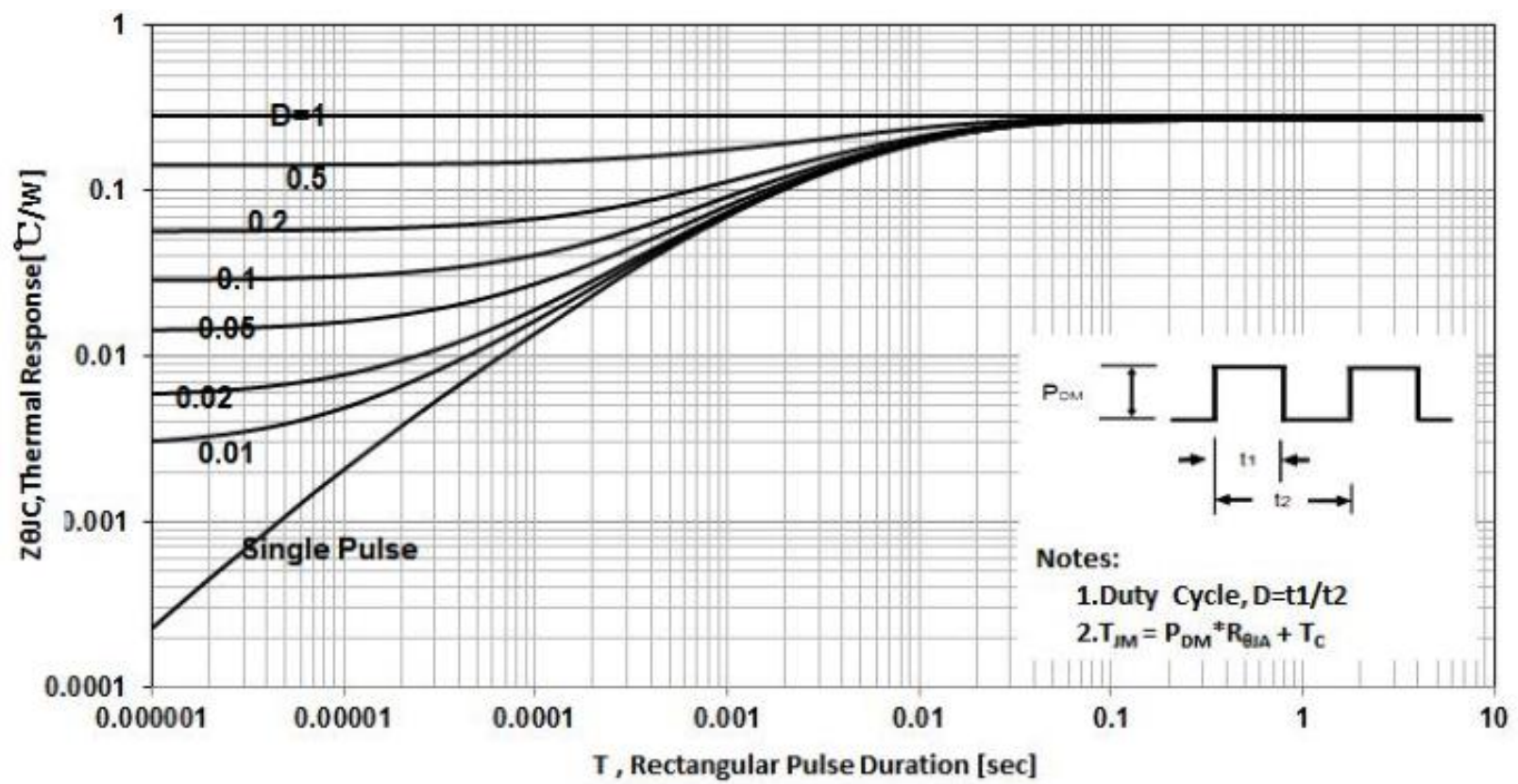
Figure 5 Maximum Effective Thermal Impedance , Junction to Case
