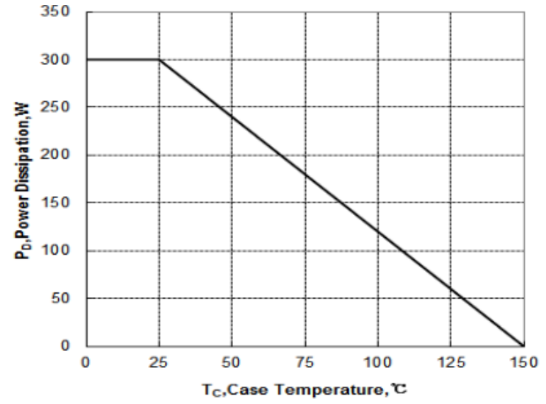
Figure 2 Maximum Power dissipation vs Case Temperature
