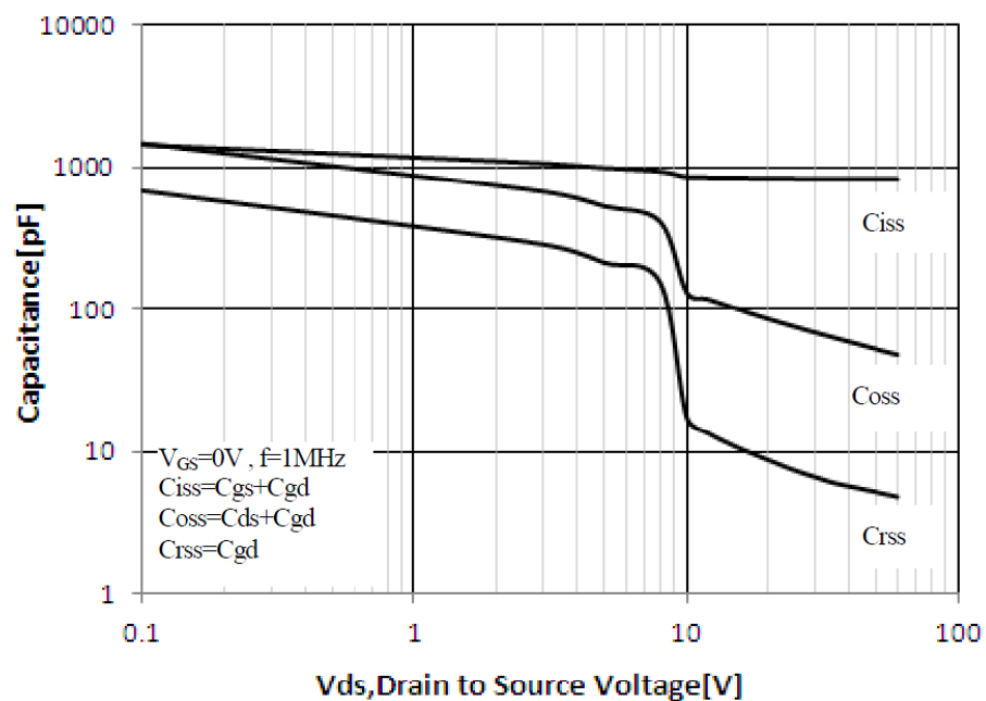
Figure 12 Typical Capacitance vs Drain to Source Voltage
