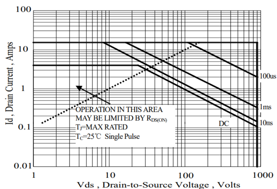
Figure 1 Maximum Forward Bias Safe Operating Area
