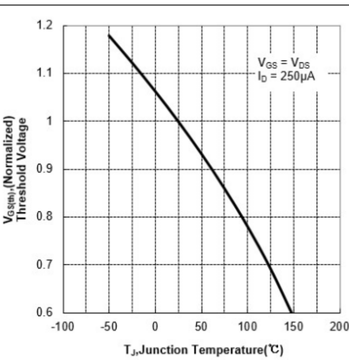
Figure 8 Typical Threshold Voltage vs Junction Temperature
