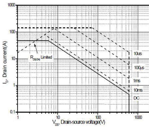
Figure 11. Safe operation area T_C = 25 \text{ °C}
