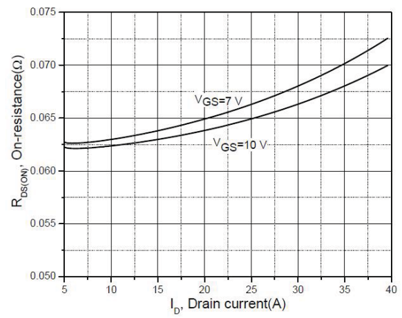
Figure 10. Drain-source on-state resistance
