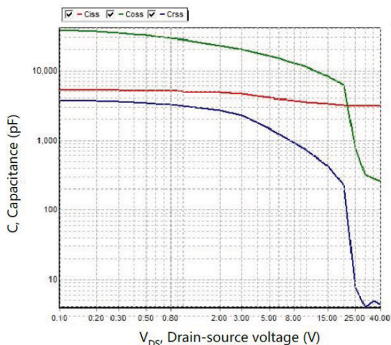
Figure 3. Typ. capacitances
