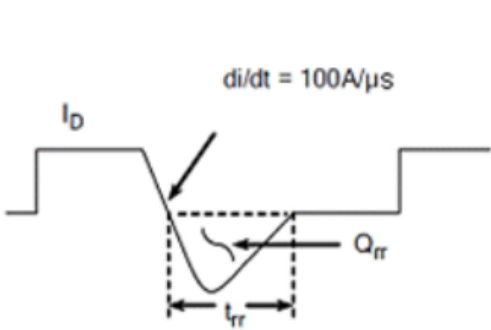
Figure 17 Diode Reverse Recovery Waveform
