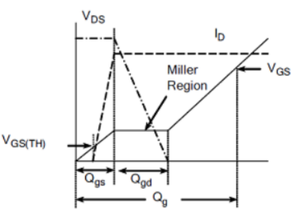
Figure 13 Gate Charge Waveforms
